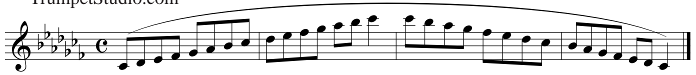
Cb Major
